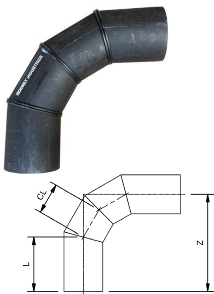
Segmented Bends - 90°
