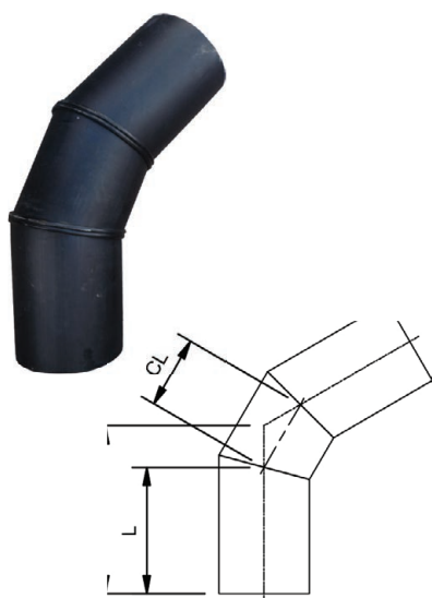
Segmented Bends - 60°
